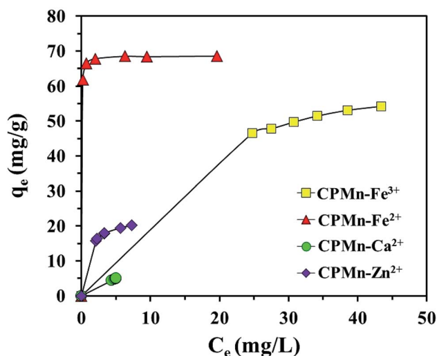
Fig. 9 The equilibrium adsorption of \text{Fe}^{3+} , \text{Fe}^{2+} , \text{Ca}^{2+} and \text{Zn}^{2+} by CPMn modified with \text{KMnO}_4 . The relative combined expanded uncertainty tSE is < \pm 0.03 \text{ mg g}^{-1} (0.95 level of confidence). The initial concentration of adsorbate ( C_0 ): \text{Fe}^{3+} = 210\text{--}260 \text{ mg L}^{-1} , \text{Fe}^{2+} = 200\text{--}250 \text{ mg L}^{-1} , \text{Ca}^{2+} = 20\text{--}30 \text{ mg L}^{-1} , \text{Zn}^{2+} = 65\text{--}90 \text{ mg L}^{-1} ; 25 mL; adsorbent amount = 0.10 g; time ( t ) = 60 min; temperature ( T ) = 303.15 K; pressure ( P ) = 101 kPa.
