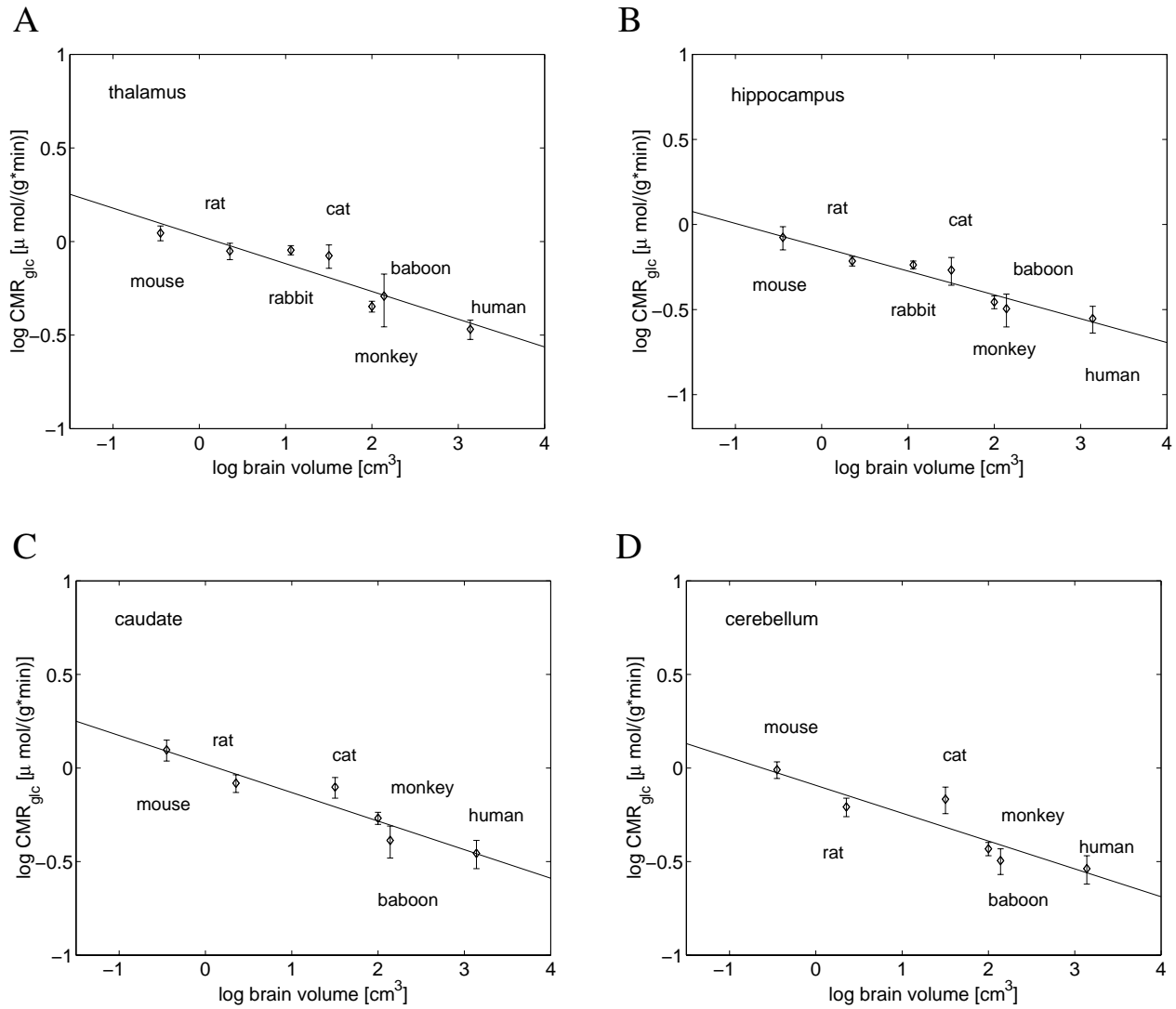
Figure 3 Scaling of the volume-specific glucose utilization rate in subcortical gray matter with brain volume. The specific metabolic scaling exponent had the following values: (A) -0.15 for thalamus ( y = -0.15x + 0.03 ); (B) -0.14 for hippocampus ( y = -0.14x - 0.13 ), which represents limbic structures; (C) -0.15 for caudate ( y = -0.15x + 0.02 ), which represents basal ganglia; (D) -0.15 for cerebellum ( y = -0.15x - 0.09 ).
