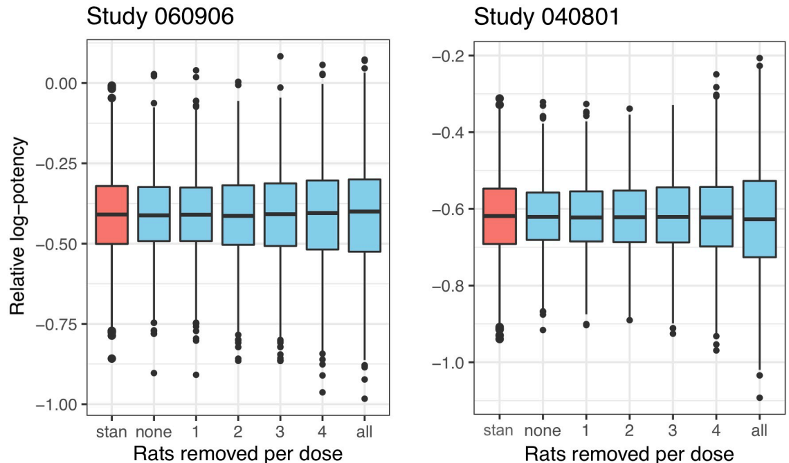
Fig 4. Box plots of the estimated relative log-potency based on 1000 simulations for the two studies. The red box indicates a re-fit using the standard approach, and the remaining blue box plots are the re-fits using the mixed-effects meta-analysis approach, removing different numbers of control rats per dose value: none and all indicate keeping and removing all the control rats, respectively, rem1 indicates removing one control rat per dose value, rem2 removing two and so on.
