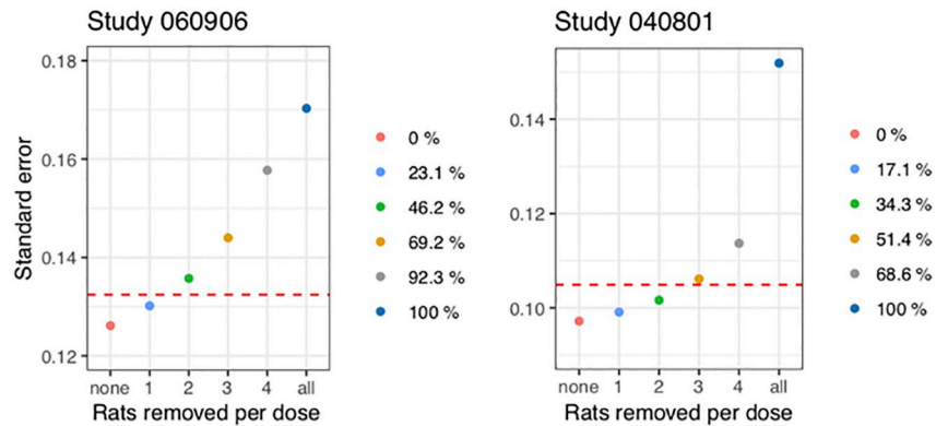
Fig 5. Standard error for the relative log-potency based on 1000 simulations for the two studies. The red dotted line is the standard error on the parameter from re-fitting the simulated data using the standard approach. The points indicate the re-fits using the mixed-effects meta-analysis approach, removing different numbers of control rats. On the x-axis, the number of control rats removed per dose is seen, and the legend shows the resulting reduction in percent of the total number of control rats.
