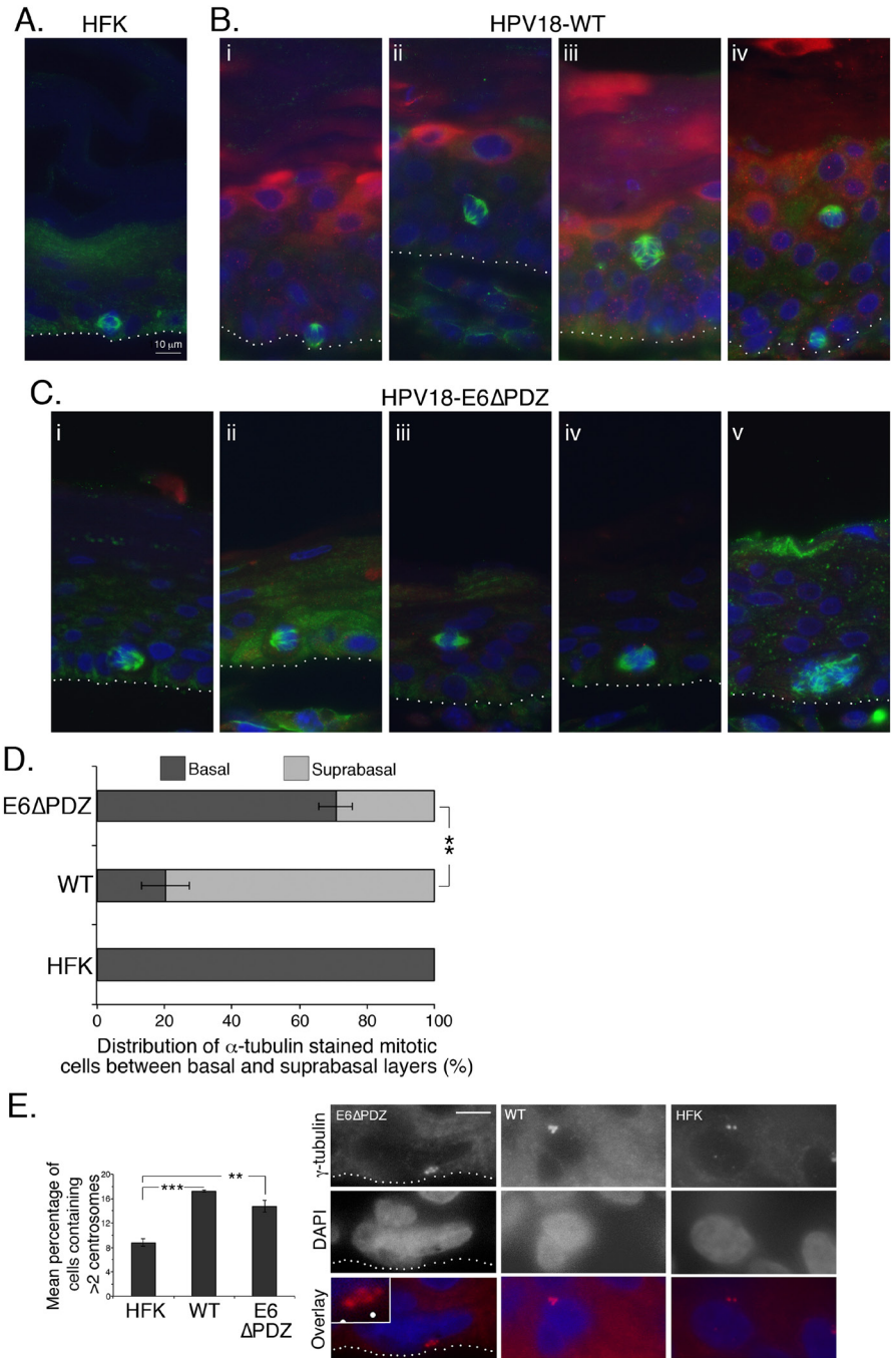
Figure 6: Loss of E6 PBM function is associated with an alteration in the distribution of \alpha -tubulin stained mitotic cells between basal and suprabasal cell layers of organotypic rafts. Sections of organotypic raft cultures of A. untransfected HFK, B. HPV18 WT genome-containing cells and C. cells containing E6 \Delta PDZ genomes, were stained for \alpha -tubulin (green), HPV18 E4 (red), and DNA (blue). Examples given in B and C were taken from multiple donors. The dotted white line in A, B and C indicates the junction between the basal cell layer and fibroblast embedded collagen matrix. D. The distribution of mitotic cells between the basal and suprabasal cell layers of organotypic rafts shown as a percentage of total \alpha -tubulin stained mitotic cells ( \pm standard error of the mean). Data were collected from three donors, and for each donor five sections of organotypic raft were analyzed (full thickness and entire length). Numbers of \alpha -tubulin stained mitotic cells counted were 47 (HFK), 525 (WT) and 230 (E6 \Delta PDZ). Student's t test was used to determine significance (**, p < 0.01 ). E. Sections were stained with \gamma -tubulin to visualize centrosomes and cells with visible centrosomes were scored for centrosome number. Rafts prepared from three different donors were analyzed; numbers of cells scored were: 1772 (HFK), 4022 (WT) and 2758 (E6 \Delta PDZ). Student's t test was used to determine significance (**, p < 0.01 ; ***, p < 0.001 ). Shown are examples of cells in E6 \Delta PDZ, WT rafts with >2 centrosomes, and an HFK raft with 2 centrosomes (red, \gamma -tubulin; blue, DAPI). The E6 \Delta PDZ centrosomes are shown enlarged in the inset and the dotted white line indicates the junction between the basal cell layer and fibroblast embedded collagen matrix. Scale, 10 \mu m (inset 18.5 \mu m).
