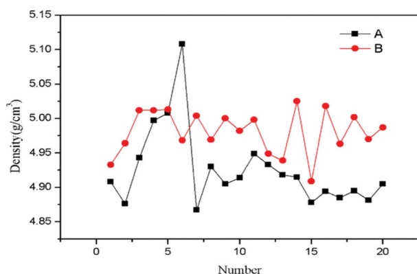
Fig. 6 Density of \text{SiO}_2@Pb/B_4C/BPRs composites in 20 regions. A: Pb/ B_4C/BPRs composites; B: 0.486 wt% \text{SiO}_2@Pb/B_4C/BPRs composites.
