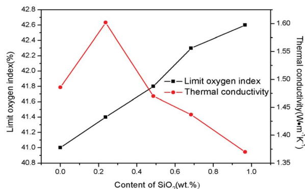
Fig. 7 LOI and thermal conductivity of \text{SiO}_2@Pb/B_4C/BPRs composites with different content of \text{SiO}_2 .
