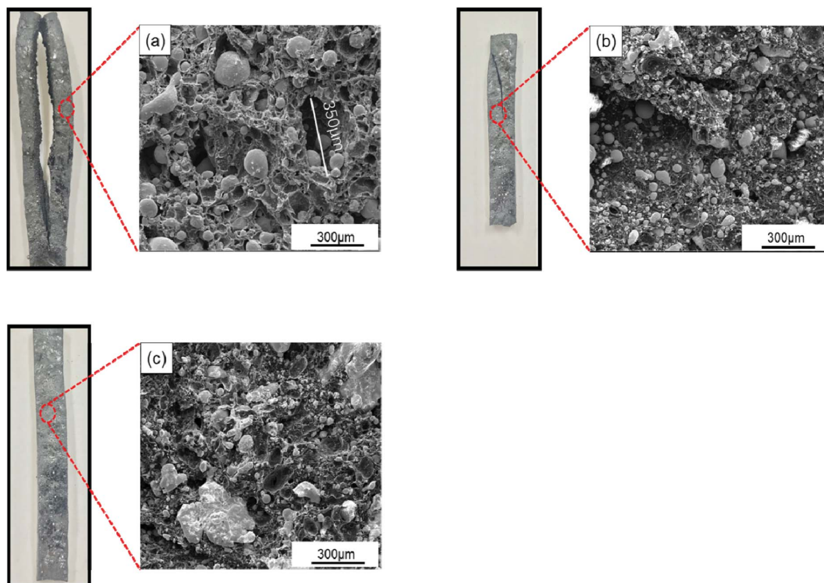
Fig. 8 Photographs and SEM images of \text{SiO}_2@Pb/B_4C/BPRs composites after burning with different content of \text{SiO}_2 : (a) Pb , (b) 0.486 wt% \text{SiO}_2@Pb , (c) 0.967 wt% \text{SiO}_2@Pb .
