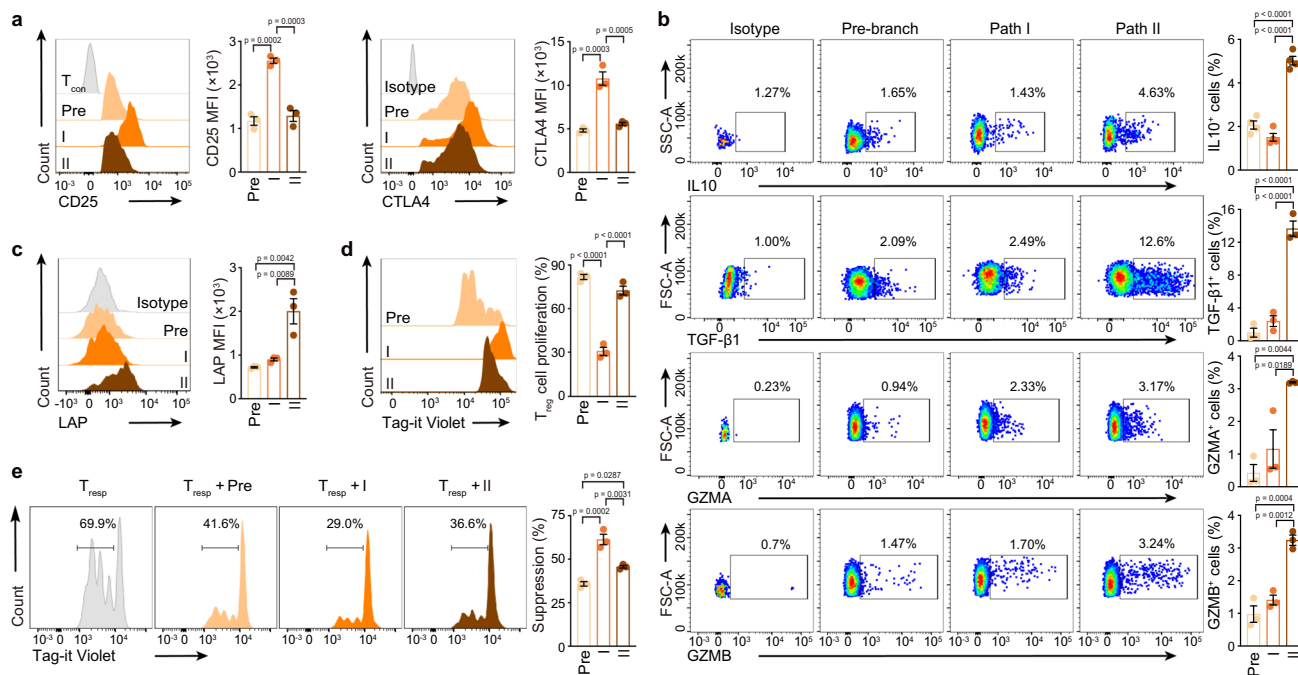
Fig. 4 In vitro assay of T reg cell paths. a–c Flow cytometry and its quantification of the indicated proteins in each HD PB T reg cell path (CD25: n = 3, CTLA4: n = 3, IL10: n = 4, TGF-β1: n = 3, GZMA: n = 3, GZMB: n = 3, LAP: n = 3). d The proliferation of HD PB T reg cell paths. The Tag-it Violet dilution of T reg cells were assessed by flow cytometry, after 96 h in vitro culture ( n = 3). e In vitro suppression assay ( n = 3). Tag-it Violet-labeled HD PB T resp cells were co-cultured with different HD PB T reg cell paths for 96 h with CD3/CD28 T cell activator. The T reg : T resp ratio was 1: 2. The Tag-it Violet dilution of T resp cells were assessed by flow cytometry. In a–e , experiment repeated at least three times; p values were determined by One-way ANOVA; data are presented as mean values ± SEM. Source data are provided as a Source Data file.
