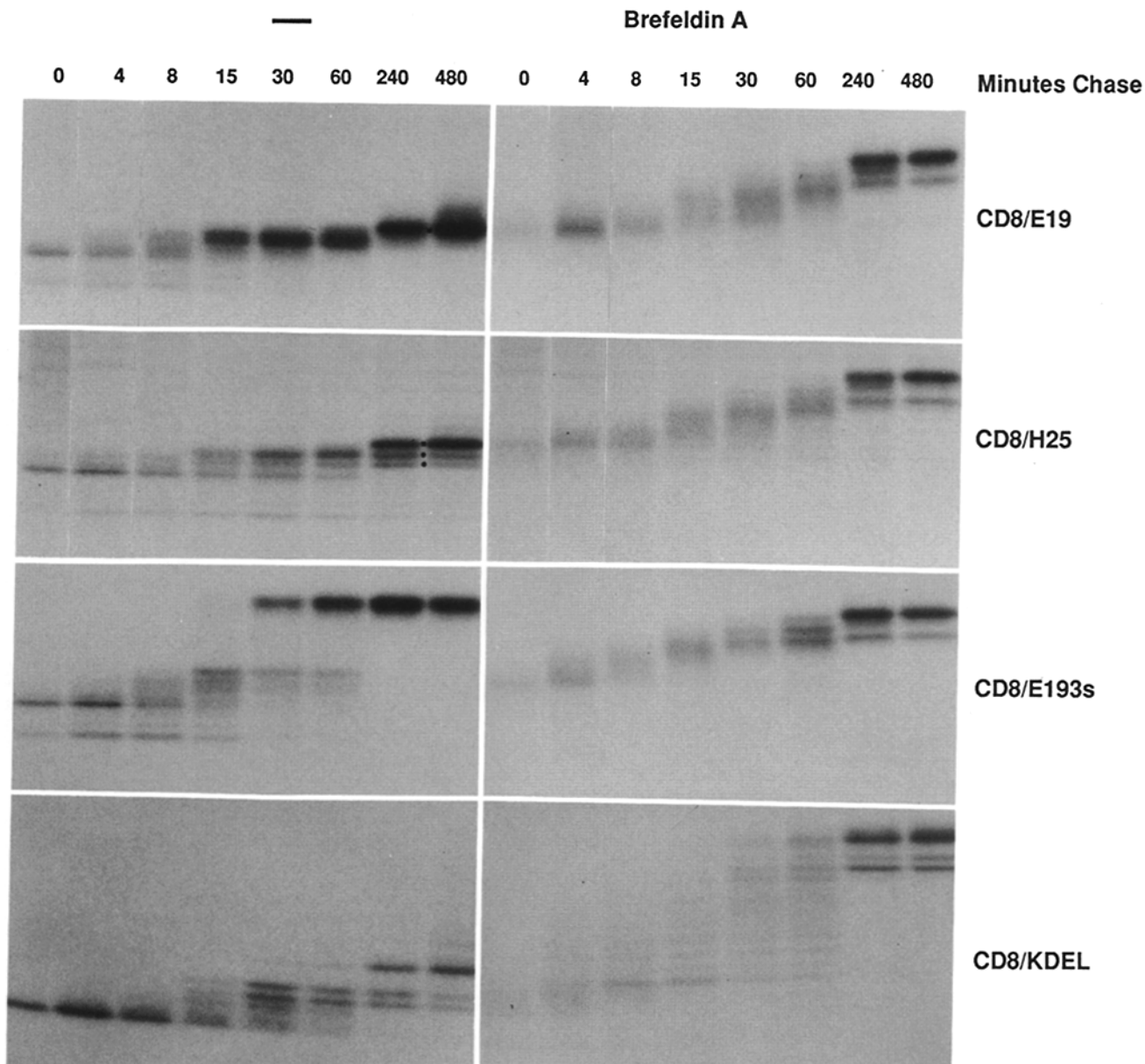
Figure 7. Post-translational modification of CD8 chimeras in cells treated with brefeldin A. HeLa cells transfected with the expression plasmids indicated in the figure were labeled for 5 min with [ 35 S]methionine and subsequently chased for the times indicated. Two series of pulse/chase plates were set up for each construct. These were treated identically except that brefeldin A (2 μg/ml) was added to one series 1 h before labeling and the drug was maintained in the labeling and chase media. The labeled CD8 proteins were collected and analyzed as described in Fig. 6. Note that due to its smaller size the various post-translationally modified forms of CD8/KDEL are better resolved on the SDS gels than the post-translationally modified forms of the transmembrane CD8 chimeras (see Fig. 1).
