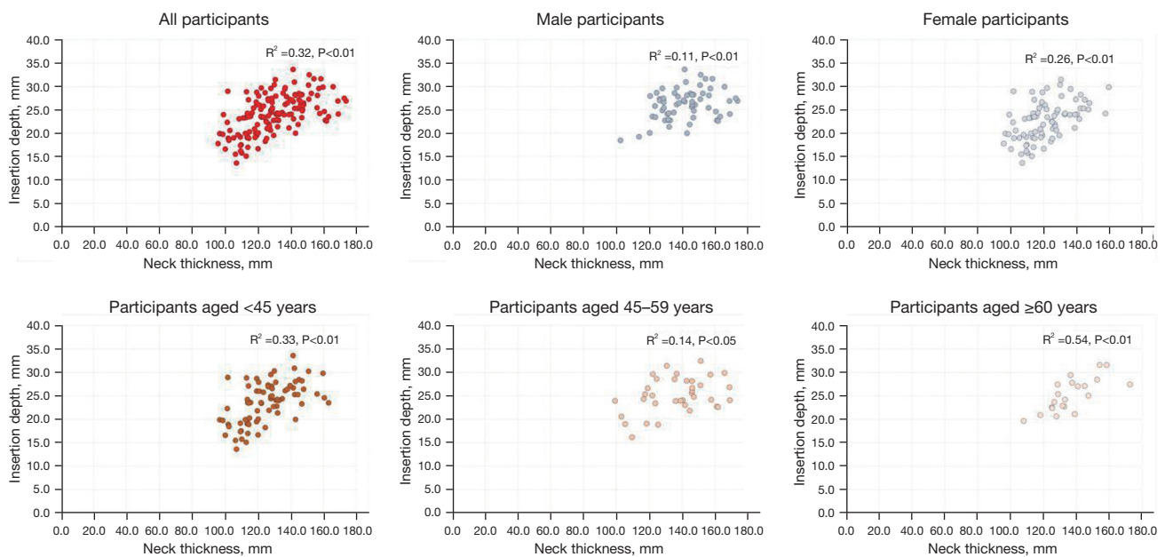
Figure 3 Results of Pearson correlations between insertion depth and neck thickness.
