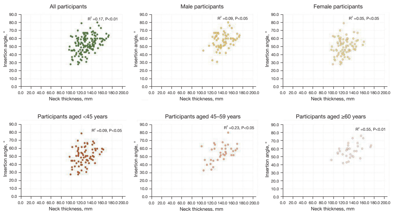
Figure 4 The Pearson correlations between insertion angle (°) and neck thickness for all participants.
