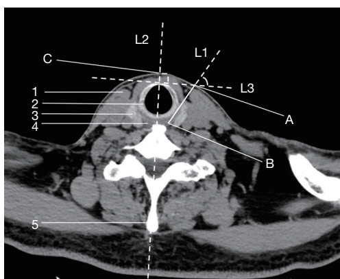
Figure 1 Measurement of the insertion angle, the insertion depth, and the distance. 1: the sternocleidomastoid muscle. 2: the cricoid cartilage. 3: the thyroid gland. 4: the cricopharyngeal muscle. 5: the cervical spine. A: the anterior border of the sternocleidomastoid muscle. B: the most superficial position of the CP muscle; L1: extension of line through A and B. L2: the line through the midpoint of the anterior border of the cricoid cartilage and the midpoint of the cervical spinous process to mark the mid-sagittal plane. L3: the straight line through the anterior border of the sternocleidomastoid muscle (point A) and perpendicular to L2.
