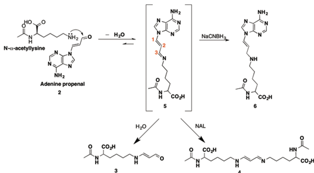
Figure 4. Proposed scheme for the reaction of adenine propenal with N -α-acetyllysine.
