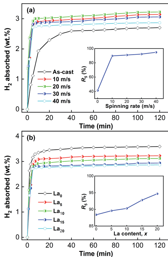
Fig. 6 Hydrogen absorption kinetic curves of the as-cast and spun ( \text{Mg}_{24}\text{Ni}_{10}\text{Cu}_2 ) 100-x La x ( x = 0-20 ) alloys: (a) \text{La}_{20} alloy, (b) as-spun alloys ( 40 \text{ m s}^{-1} ).
