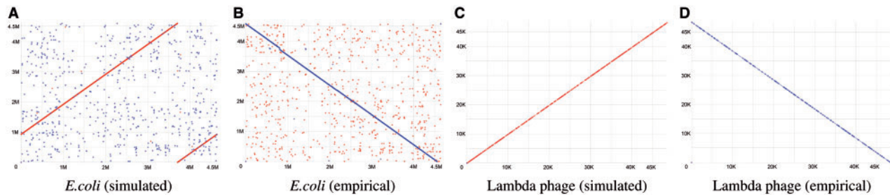
Fig. 8. Mummer plots comparing the reference genome on the x-axis with the assembled genome on the y-axis. (A) The assembly result of the E.coli K-12 genome by Canu, using simulated reads from DeepSimulator. (B) The assembly result of the E.coli K-12 genome by Canu, using the experimental MinION sequence data (i.e. empirical data). (C) The assembly result of the lambda phage genome by Miniasm with Racon, using simulated reads from DeepSimulator. (D) The assembly result of the lambda phage genome by Miniasm with Racon, using the empirical data
