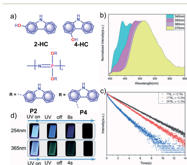
Fig. 10 (a) Chemical structure of monomers 2-HC and 4-HC , and polymers P2 and P4 . (b) Excitation wavelength-dependent phosphorescence spectra and (c) temperature-dependent phosphorescence decay curves of PVA-100-P4-1 film. (d) Photographs of persistent luminescence of PVA-100-P4-1 film under ambient conditions. Reproduced with permission from ref. 112. Copyright 2020, WILEY-VCH.
