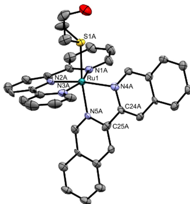
Fig. 2 Displacement ellipsoid (50% probability level) of one crystallographically independent cationic part as observed in the crystal structure of [2]^{2+} . The other cation, disorder, counter ions, and H atoms have been omitted for clarity
