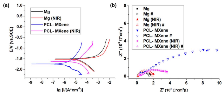
Fig. 8 Electrochemical corrosion analysis of the effect of NIR on bare Mg and PCL-MXene coating on Mg, (a) potentiodynamic polarization measurement of each group and (b) raw data and fitting results (#) of each group Nyquist plots.
