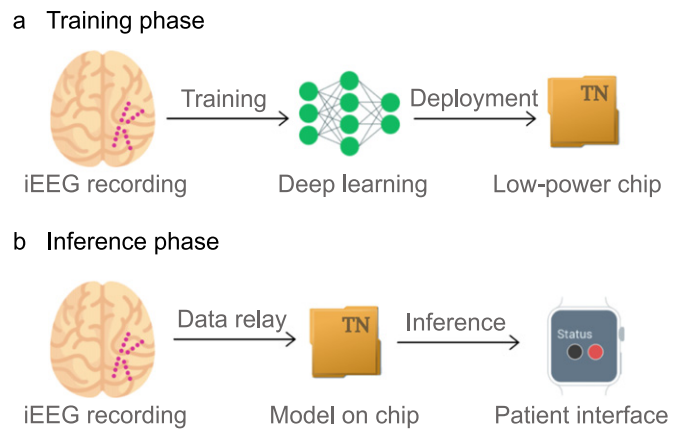
Fig. 1. Concept of seizure advisory system: a) Training phase: iEEG signal is recorded via intracranial electrodes (magenta circles indicate a possible configuration) and recordings are passed on to a deep learning network (green network graph). The model is subsequently deployed onto a TrueNorth chip. b) Inference phase: iEEG signal is recorded via intracranial electrodes (magenta circles) and recordings are passed on to the TrueNorth chip. Prediction of a seizure is indicated to the patient on a wearable device.
