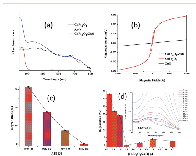
Fig. 6 DR-UV-Vis diffuse reflectance spectra (a) and magnetic studies (b) of the various nanocatalysts synthesized using low-frequency ultrasound; percentages of degradation of Acid Blue 113 at various concentrations in the presence of a fixed \text{CoFe}_2\text{O}_4/\text{ZnO} nanocatalyst dosage ( 1.5 \text{ g L}^{-1} ) (c); and percentages of degradation of Acid Blue 113 [ 5 \times 10^{-5} M] in the presence of various dosages of \text{CoFe}_2\text{O}_4/\text{ZnO} (d). The insert shows the observed characteristic changes in the UV-Vis spectra of AB113 degradation.
