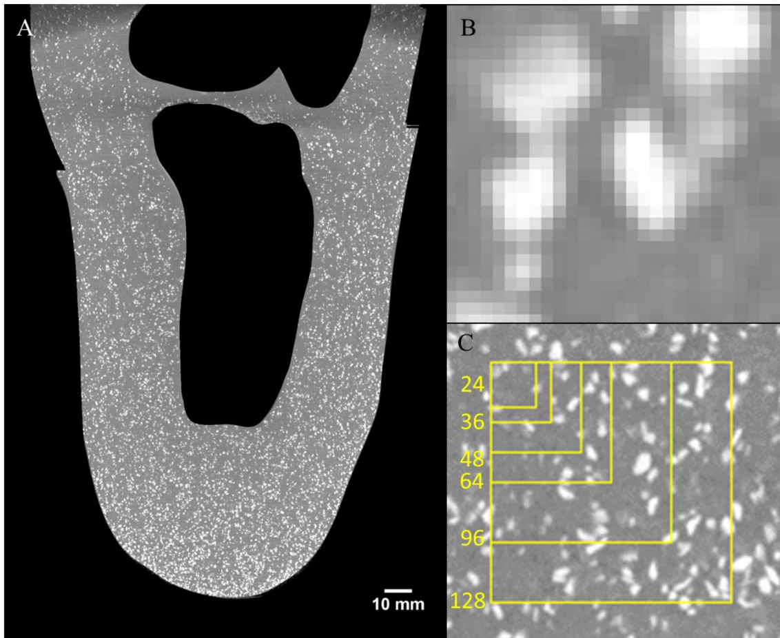
Figure 3. Example reconstructed CT section of a sagittal plane through the model, with bones and surrounding areas masked (A), magnified view of sand particle features compared to the 108 \mu\text{m} -cube voxels (B), and comparing subvolume size (yellow squares) from 24 to 128 voxels (2.6 to 13.8 mm) squares (C).
