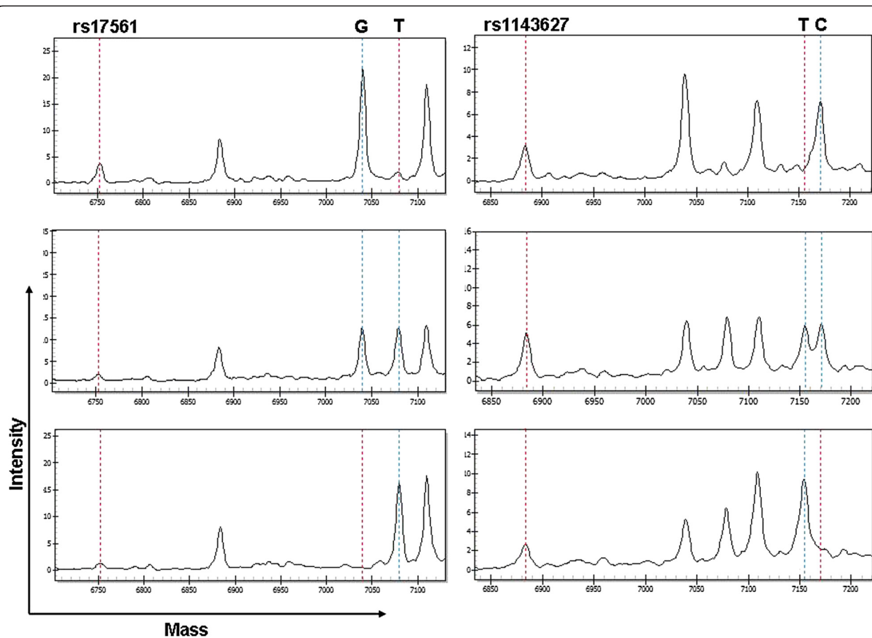
Figure 2 MALDI-TOF mass spectrometry-based analysis of rs17561 and rs1143627 SNPs. Typical MALDI-TOF MS spectra from three DNA samples are shown. Dashed lines mark the unextended primers and product/extended primers. Rs17561 SNP includes GG, GT, and TT genotypes, and rs1143627 SNP includes CC, TC, and TT genotypes.
