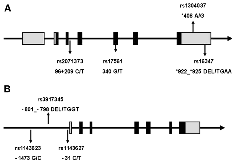
Figure 1 Schematic representation of IL-1 \alpha and IL-1 \beta genes. (A) is IL-1 \alpha and (B) is IL-1 \beta gene. The boxes represent the exons. The black boxes represent coding sequences and grey boxes represent 3' or 5' untranslated regions. SNPs analyzed in this study are marked with an arrow. The first line following the direction of arrow marking the SNPs shows the SNP name (i.e. rs-number) from NCBI, and the second line shows the SNP position and the base substitution starting from the start codon.
