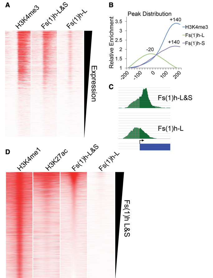
Figure 3. Sites of Fs(1)h-S correlate with gene expression and show a different binding profile than Fs(1)h-L. (A) TSSs were sorted by expression level from highest to lowest and given up/downstream orientation according to strand. The total number of reads is plotted for each ChIP-seq data set in 20 bp bins covering 1 kb upstream and downstream from each TSS and viewed in Java Treeview. (B) Peaks unique to Fs(1)h-S and Fs(1)h-L data sets present around TSSs were plotted in 20 bp bins, and the average profile was plotted covering 200 bp upstream and downstream from the TSS and compared with the average profile of H3K4me3. Read counts within the window were normalized to the total reads within the window and plotted as a fold enrichment over the baseline calculated, as the average number of reads across the window to compare between data sets. (C) Example of a gene with an Fs(1)h-L&S peak shows that the Fs(1)h-L summit is found slightly upstream of the TSS, and the Fs(1)h-S summit is found slightly downstream of the TSS but still has enrichment upstream from the Fs(1)h-L cross-reactivity. (D) Enhancers identified by H3K4me1 enrichment were used as anchors around which the total number of reads is plotted for each ChIP-seq data set in 20 bp bins covering 1 kb upstream and downstream. The enrichments were then sorted by Fs(1)h-L&S intensity and viewed in Java Treeview.
