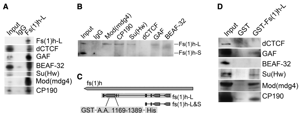
Figure 6. Fs(1)h-L interacts with insulator proteins. (A) Co-IP experiments with a protein lysate from Kc167 cells (Input) were performed using either IgG (control) or antibody against Fs(1)h-L (guinea pig). Western analysis was performed on all samples using antibodies designated on the right side of the panel at 1:10 volume of input to IP. (B) Co-IP experiments were performed as described earlier in the text with only one immunoprecipitation from the lysate using antibodies against each of the indicated insulator proteins followed by western blotting with Fs(1)h antibodies that recognize both isoforms. (C) Organization of the Fs(1)h locus. Amino acids 1169 through 1389 were placed in an expression vector with a GST tag at the N-terminus and His 6 tag at the C-terminus for expression in E. coli followed by purification to 1.3 μg/μl using the His 6 and GST tags. (D) The Fs(1)h-L specific peptide was incubated with a Kc cell protein lysate, precipitated with glutathione-agarose beads and analyzed by western blot to test for interaction with each of the insulator proteins. Results suggest that GAF, Su(Hw), CP190 and Mod(mdg4) interact, directly or indirectly, with the CTM domain of Fs(1)h-L.
