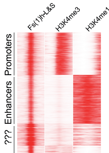
Figure 1. Fs(1)h is found at enhancers and promoters. ChIP-seq data for Fs(1)h-L&S, H3K4me3 and H3K4me1 \pm 1 kb from each peak summit was K-means clustered using Cluster 3.0 and viewed in Java Treeview. Promoter regions contain H3K4me3 but lack H3K4me1, whereas enhancer regions are marked by the presence of H3K4me1 and absence of H3K4me3. Fs(1)h-L&S is present at enhancers and promoters. In addition, a subset of sites indicated by question marks at the bottom of the heatmap is present in regions of the genome of unknown function.
