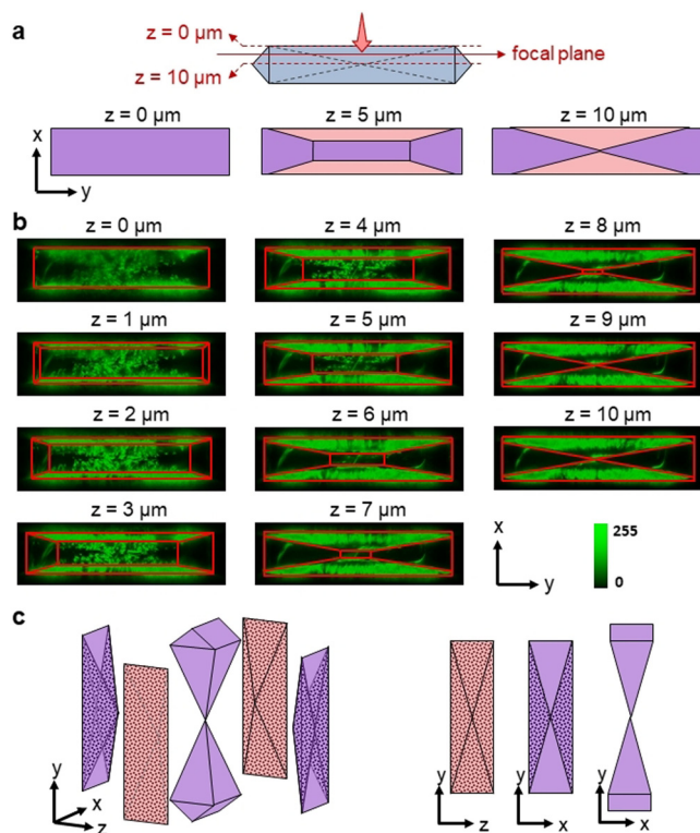
Figure 2. a) confocal xy-raster scanning of ZSM-5 (roof view) at different z-heights by moving the focal plane from z=0–10 μm (Δz=1 μm). xy-cuts at z=0, 5 and 10 μm show intersection of focal plane with crystal subunits. Color code is identical as in Figure 1; b) xy-maps at z=0–10 μm; subunit boundaries are indicated as red lines; c) 3D representation of the volume parts of ZSM-5 which develop hierarchical porosity during desilication (left, dotted areas represent hierarchical pore regions); 2D projections (right).
