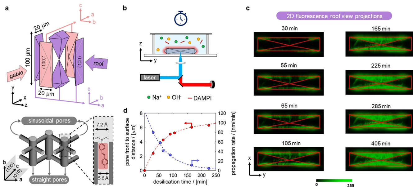
Figure 1. a) Subunit structure and micropore orientation of ZSM-5. DAMPI fluorescent dye narrowly fits in straight channel (5.6 Å), while its terminal diethylamino-group (7.2 Å) blocks further intrusion into the micropore. b) in situ fluorescence microscopy to monitor desilication by mixing ZSM-5 in a reaction cell with 0.2 M NaOH solution containing DAMPI. The laser raster scans a ZSM-5 crystal (roof view). c) 2D in situ fluorescence projections (roof view) averaged over the z-heights of the crystal during hierarchical porosity formation. d) pore front position relative to the external surface of gable pyramidal subunits (left axis) and propagation rate of pore formation (right axis) vs. desilication time.
