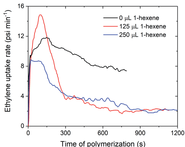
Fig. 4 Slurry-phase polymerisation ethylene uptake rate as a function of time of polymerisation using sMAO supported Me 2 SB( t BuN,I*)TiCl 2 (1 sMAO ) with 0 (black), 125 (red), and 250 μL 1-hexene (blue). Polymerisation conditions: 8.3 bar ethylene, 0.20 mg pre-catalyst ([Al] sMAO /[Ti] 0 = 200), 5.0 mL heptane, 10 μmol TiBA, and 80 °C. Reactions quenched at 5.5 bar ethylene uptake or after 60 minutes.
