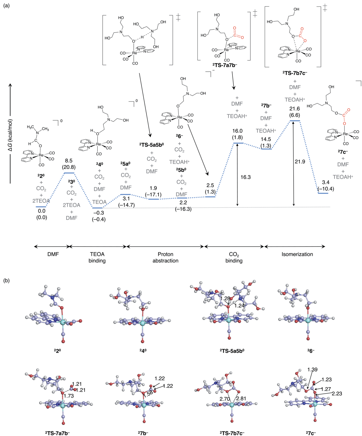
Fig. 6 (a) The free energy profile for the formation of the monoalkyl carbonate complex starting from the one-electron-reduced complex. \Delta G and \Delta H (in parentheses) are given in \text{kcal mol}^{-1} . (b) Optimized key stationary points with the selected bond distances ( \text{\AA} ). The blue bars represent one-electron-reduced doublet Re complexes.
