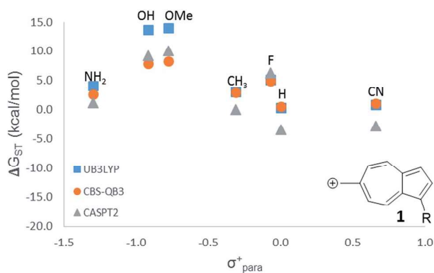
Fig. 1 LFER comparing the three methods used in this study. (■) UB3LYP/6-31+G(d,p) (corrected singlet) (●) CBS-QB3 (▲) CASPT2/ANO-L-VTZP//CBSB7.
