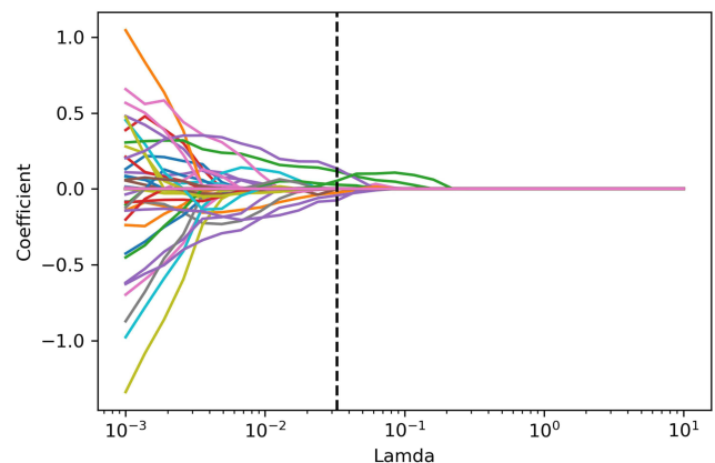
Figure 4 The values of the coefficients and the corresponding lambda values, each curve represents each feature in the model.
