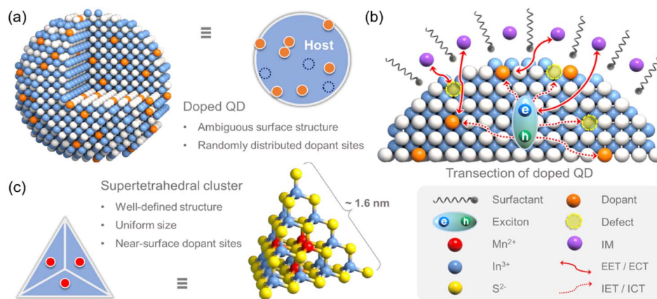
Scheme 1 (a) Schematic of a classical QD with randomly distributed dopant/defect sites. (b) Transection of a doped QD showing IET/ICT from the host to the dopant (or defect) and EET/EET between the host (or dopant/defects at different sites) and IMs. (c) Structure of the atomically precise semiconductor model, namely, supertetrahedral T4-Mn clusters with Mn 2+ ions uniformly distributed in the near-surface region (IET, internal energy transfer; ICT, internal charge transfer; EET, external energy transfer; ECT, external charge transfer; IM, interfacial molecule).
