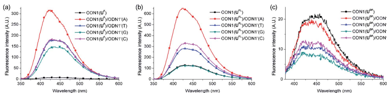
Fig. 2 Fluorescence spectra of probes featuring T-FBs, recorded in 10 mM Tris–HCl buffer (pH 7.2; 100 mM NaCl, 20 mM MgCl_2 ): ssODN1s and their duplexes (each concentration: 1.5 \mu M) formed between (a) ODN1( U^F )/ODN1'(N), (b) ODN1( U^{FL} )/ODN1'(N) and (c) ODN1( U^{DF} )/ODN1'(N); N = A, T, G or C. Excitation wavelength: absorption maximum.
