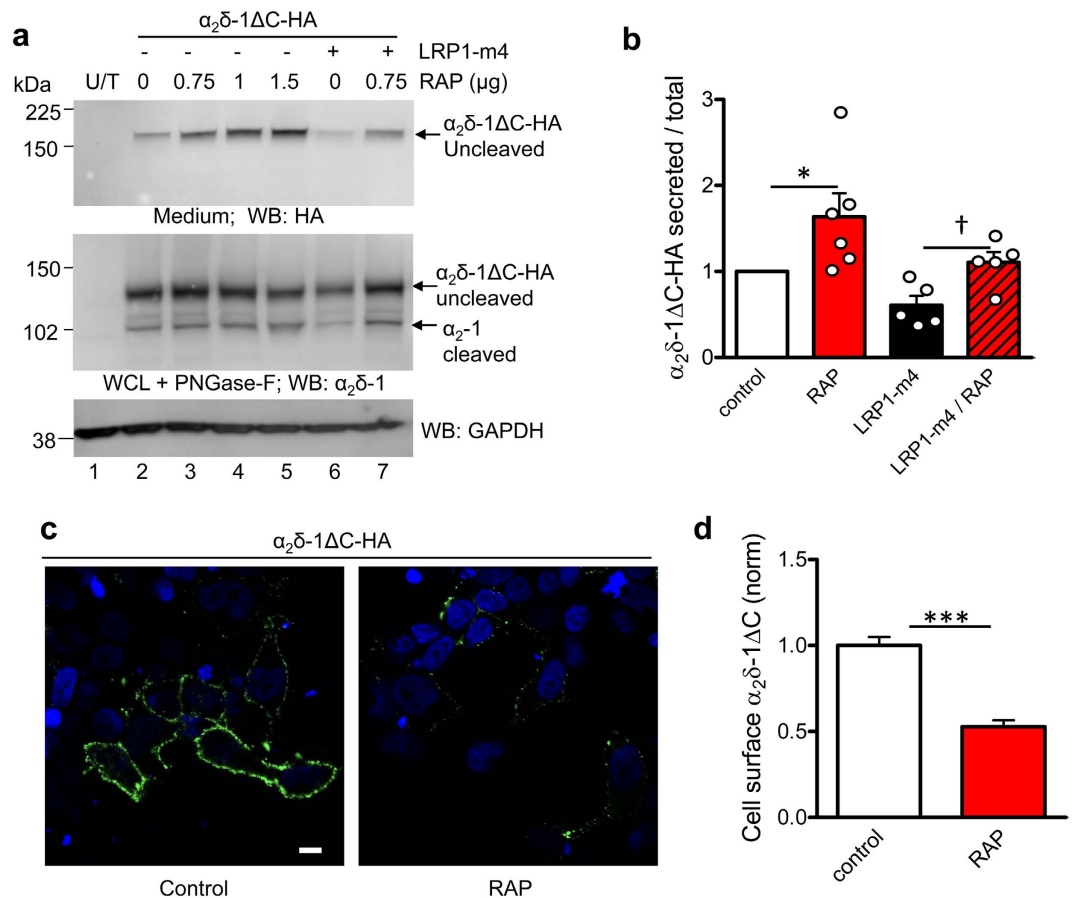
Figure 6. Effect of LRP1-m4 and RAP on secretion of anchorless \alpha_2\delta-1\Delta C . (a) \alpha_2\delta-1\Delta C\text{-HA} was expressed in tsA-201 cells either with the empty vector (lane 2) or with increasing concentrations of RAP (lanes 3–5), or with Flag-LRP1-m4 (lane 6) or Flag-LRP1-m4 plus RAP (lane 7). Lane 1 shows untransfected cells (U/T). Top panel: \alpha_2\delta-1\Delta C\text{-HA} detected in medium (HA Ab). Middle panel: \alpha_2\delta-1\Delta C\text{-HA} in WCL, deglycosylated with PNGase-F ( \alpha_2\delta-1 Ab). Note also the increase in cleaved \alpha_2-1 as RAP is increased (middle panel; lanes 2–5). Bottom panel: GAPDH loading control for WCL. (b) Quantification of experiments including that shown in (b), of \alpha_2\delta-1\Delta C\text{-HA} secreted into the medium, measured as ratio of WCL \alpha_2\delta-1\Delta C , and normalised to control without RAP in each experiment (open bar, n = 6 ), for co-transfection with RAP (0.75 \mu\text{g} ; red bar, n = 6 ), with Flag-LRP1-m4 alone (black bar, n = 5 ) or LRP1-m4 plus RAP (0.75 \mu\text{g} ; red hatched bar, n = 5 ). Data are mean \pm SEM with individual data points, * P = 0.0313 , Wilcoxon's matched pairs signed rank test compared to normalised control; † P = 0.0234 , paired t test. (c) Non-permeabilised tsA-201 cells, transfected with \alpha_2\delta-1\Delta C\text{-HA} , and cell surface-labelled with HA Ab, merged with DAPI staining. Left: control, transfected with \alpha_2\delta-1\Delta C\text{-HA} and empty vector; right: \alpha_2\delta-1\Delta C\text{-HA} co-transfected with 0.75 \mu\text{g} RAP. (d) Bar chart (mean \pm SEM) showing effect of RAP (red bar, n = 150 ), normalised to control \alpha_2\delta-1\Delta C\text{-HA} cell surface expression (open bar, n = 187 ), for n = 3 independent experiments. *** P < 0.001 , Student's t test. Full blots for all figure parts are shown in Supplementary information.
