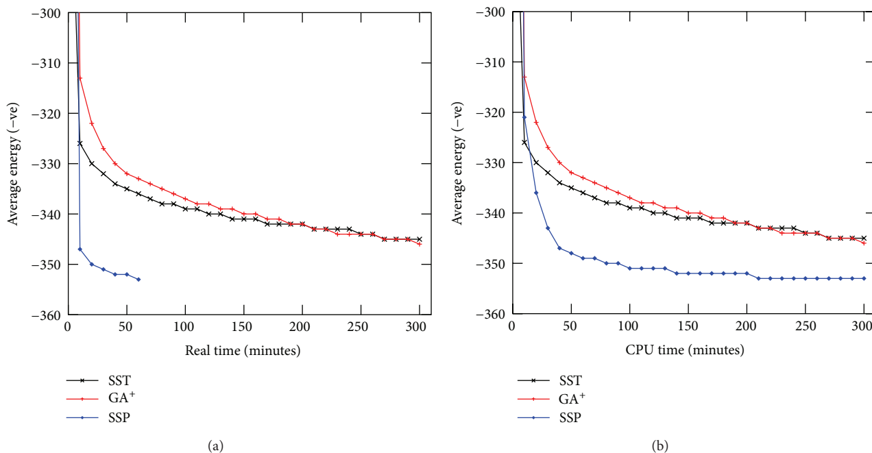
FIGURE 5: Search progress for protein RI with (a) real time and (b) CPU time of 4 threads (4x real time). SST, GA + , and SSP represent tabu-based spiral search [9], genetic algorithms [8], and multipoint parallel spiral search, respectively.
