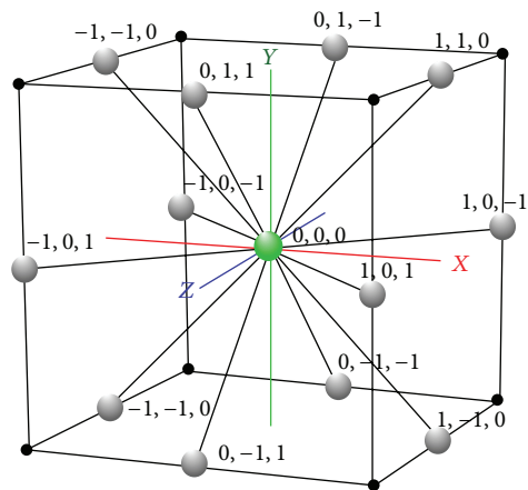
FIGURE 1: A unit 3D FCC lattice with 12 basis vectors on the Cartesian coordinates.
