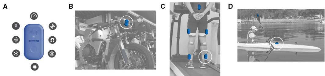
Figure 1 (A) Inertial measurement unit's applications in sports. Analyses in (B) speed motorcycling: pilot's internal and external loads, (C) running: multidevices external load running and (D) canoeing: stroke mechanic and canoe oscillation.
