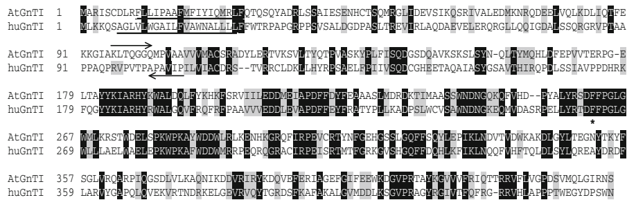
Fig. 1 Alignment of the GnTI protein sequences derived from Arabidopsis thaliana (AtGnTI) and human (HuGnTI), using ClustalW. Identical and similar residues are shaded black and grey respectively. The N-glycosylation consensus site of A.
