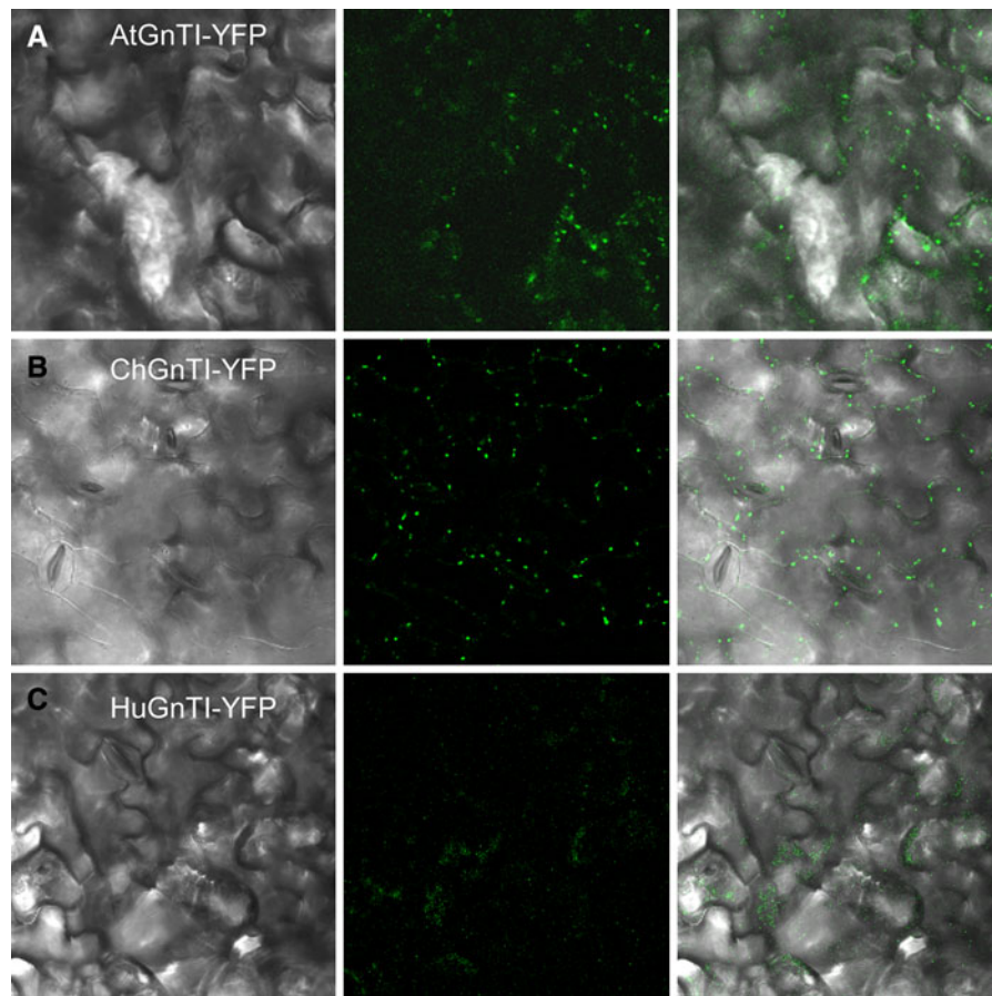
Fig. 5 Localization of the GnTI-YFP fusion proteins in leaves of 10 day old transgenic T2 seedlings by whole mount microscopy. Left : light images leaf surface. Middle : fluorescent images taken under equal filter and exposure settings. Right : overlay light and fluorescent images. Seedlings expressing AtGnTI-YFP or ChGnTI-YFP, displayed a punctate
