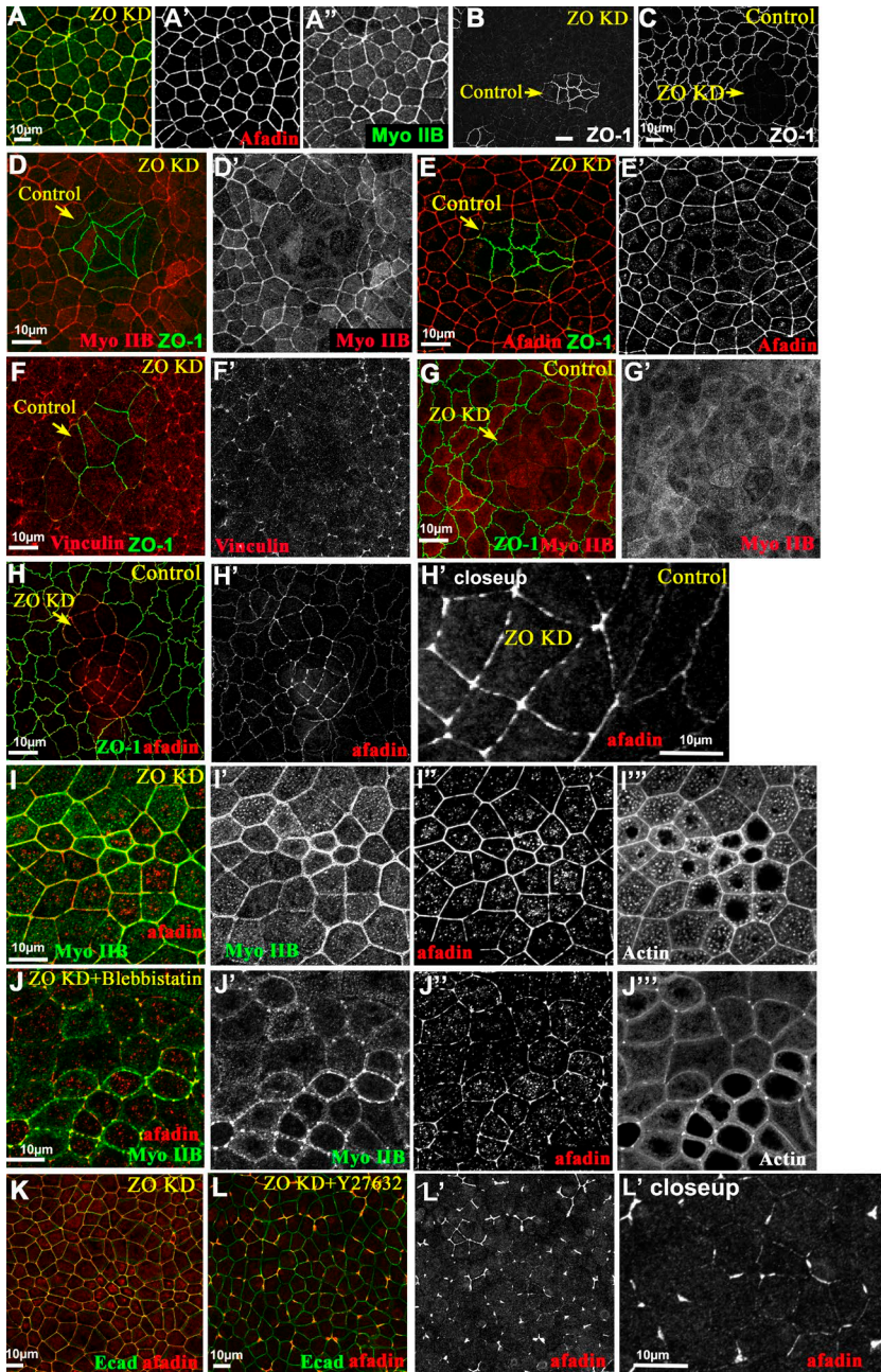
Figure 9. Feedback from tissue-level contractility and myosin activity is required for myosin accumulation but not afadin recruitment. Control, ZO KD, or mixed culture projections of apical 3- \mu m sections. Some cells treated with DMSO (control; A, I, and K); 0.1 mM blebbistatin (J); or 50 \mu M Y27632 (L). (B and D–F) Small islands of control cells in ZO KD monolayers. Each cell type retained patterns of myosin (D), afadin (E), and vinculin (F) seen in unmixed monolayers (e.g., A). (C, G, and H) Small islands of ZO KD cells in control cell monolayers. ZO KD cells had reduced cortical myosin (G), whereas afadin remained elevated cortically but became less continuous (A vs. H'). (I and J) Blebbistatin fragmented cortical myosin and afadin (I vs. J). (K and L) ROCK inhibition also made afadin more discontinuous.
