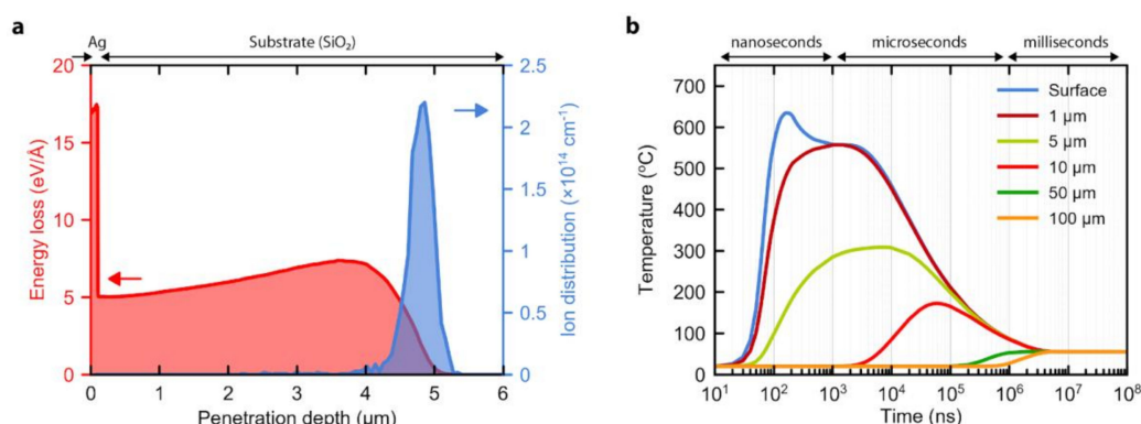
Figure 1. (a) Protons energy loss (left, y -axis) and distribution (right, y -axis) within the sample. (b) Intense pulsed ion beam irradiation induced heat transfer in Ag/SiO _2 structure, showing near-surface annealing capability.
