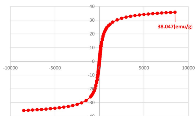
Fig. 10 VSM analysis of Fe 3 O 4 @AMBA-CuI nanocatalyst after 6 runs.
