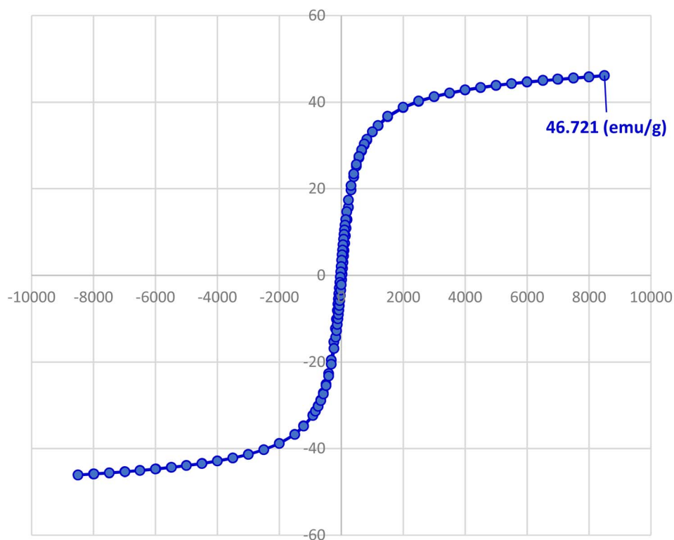
Fig. 8 VSM analysis of \text{Fe}_3\text{O}_4@AMBA\text{-CuI} nanocatalyst.
