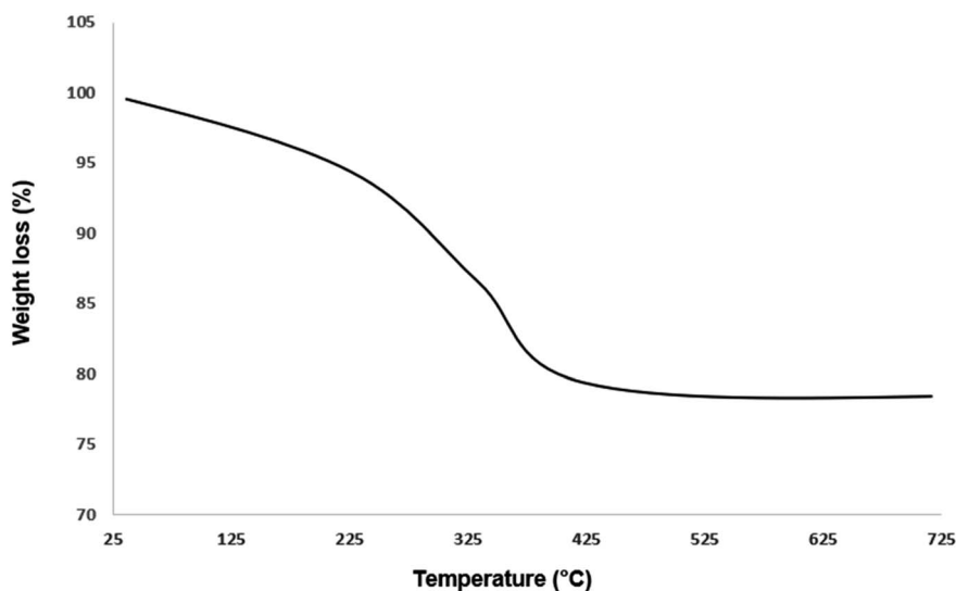
Fig. 7 TGA analysis of \text{Fe}_3\text{O}_4@AMBA\text{-CuI} nanocatalyst.
