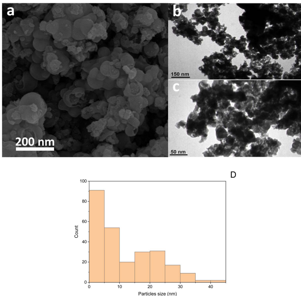
Fig. 3 (a) SEM, (b and c) TEM images of \text{Fe}_3\text{O}_4@AMBA\text{-CuI} nanocatalyst at different magnifications and (d) particles distribution histogram.
