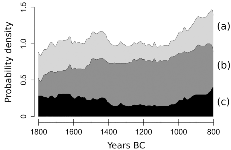
Fig 5. SCPDs of pre-screened radiocarbon dates from the EUBAR database, juxtaposed curves: (a) 1233 dates from the filtered dataset; (b) 852 14 C dates from settlements; (c) 283 14 C dates from funerary contexts (IntCal13 calibration curve).
