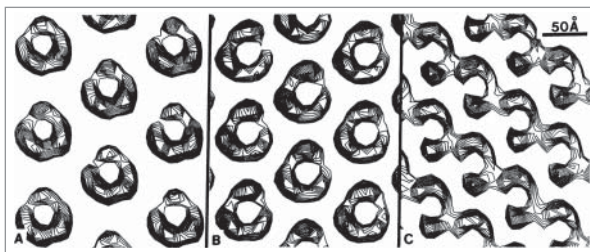
Figure 2. Filtered projection views of membrane-bound AcChoR pentameric oligomers displayed as density contour maps. The maps clearly show an aperiodic crystalline configuration. (A) Reconstructed from the structurally better preserved A surface of the tube. The stain-filled groove faces to the left for 5 of 7 tubes. (B) Reconstructed from the A surface of the tube. The groove faces to the right for 2 of 7 tubes. (C) Reconstructed from the more distorted B surface of the tube. All images are oriented such that the tube axis is vertical. The a lattice direction is always parallel to the tube axis; the b lattice direction is 125 degrees clockwise from a in A and B and is 132 degrees counterclockwise from a in C. From ref. 9 and used with permission.
