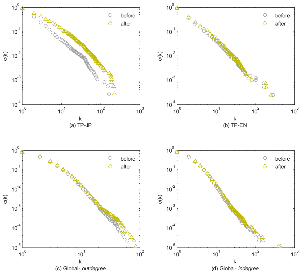
Figure 3 | Cumulative degree distribution for the extracted networks.
