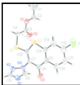
Fig. 1. The molecular structure of (I), with the atom-numbering scheme. Displacement ellipsoids are drawn at the 50% probability level.
