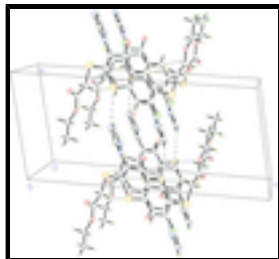
Fig. 2. A packing diagram of (I). Intra- and inter-molecular interactions are shown as dashed lines.
