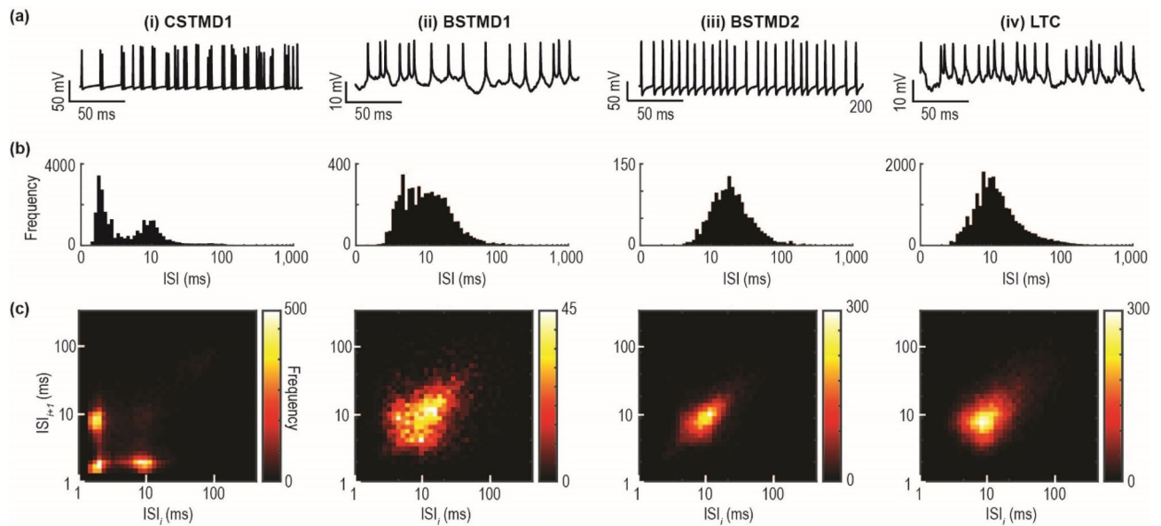
Figure 1. Statistics of spiking activity in dragonfly visual neurons. (a) Raw intracellularly recorded spike trains from 4 different dragonfly visual neurons during the presentation of a visual stimulus. (b) The distribution of ISI values from an individual example of each visual neuron. (c) The next interval ( ISI_{i+1} ) plotted as a function of the previous interval ( ISI_i ) for each neuron.
