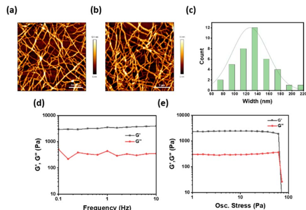
Fig. 2 AFM images of (a) ( 5/15\ \text{mM} ) \text{YCh} gel. (b) 500\ \mu\text{M} \text{Eu}^{3+} doped ( 5/15\ \text{mM} ) \text{YCh} gel. (c) Width distribution analyses of the \text{YCh} gel fibers from AFM images (number of bundled fibers counted for width distribution analyses 50). Rheology for ( 5/15\ \text{mM} ) \text{YCh} hydrogels (d) frequency sweep at fixed stress of 1.0\ \text{Pa} , (e) Stress sweep at a fixed frequency of 1.0\ \text{Hz} at 298\ \text{K} .
