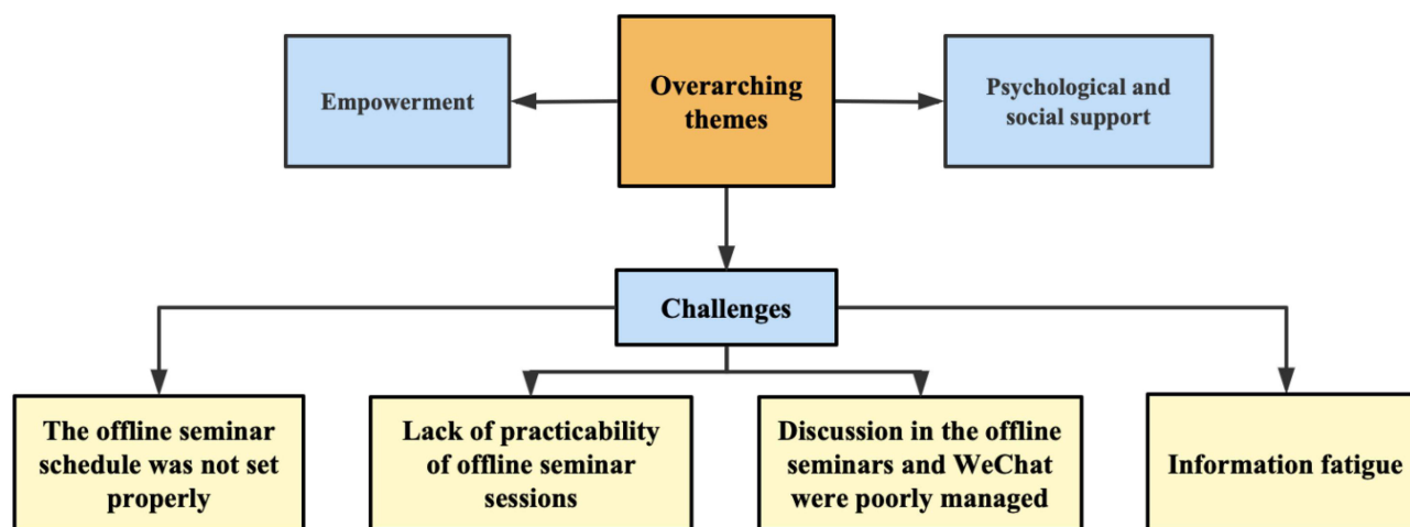
Figure 2 Overarching themes.
