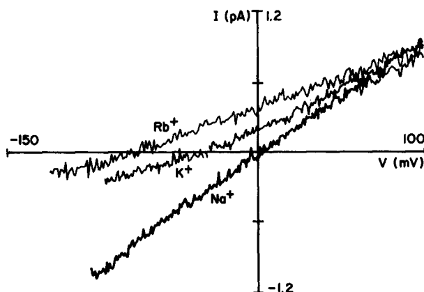
FIGURE 3. VT-activated channels are \text{Na}^+ selective. Open channel I - V curves were measured by the voltage-ramp method under bi-ionic conditions, with 200 mM \text{Na}^+ solution on the internal side of the bilayer, and 200 mM \text{Na}^+ , \text{K}^+ , or \text{Rb}^+ solutions, as indicated, on the external side. The reversal potentials are reported in Table I.
