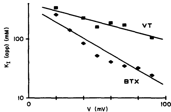
FIGURE 11. Voltage dependence of \text{Na}^+ channel block by \text{K}^+ . The apparent inhibition constants of \text{Na}^+ currents by \text{K}^+ were calculated as a function of applied voltage from data as in Fig. 10, with VT (squares) or BTX (diamonds) as the activator. The data were compiled from \geq 10 bilayers in the presence of either activator. The straight lines were the best fit of a linear regression analysis. The slopes of these lines give an e-fold increase in affinity of \text{K}^+ block per 67 mV for VT and per 31 mV for BTX. Zero-voltage inhibition constants are similar for both activators (420 mM for VT-modified and 350 mM for BTX-modified \text{Na}^+ channels).
