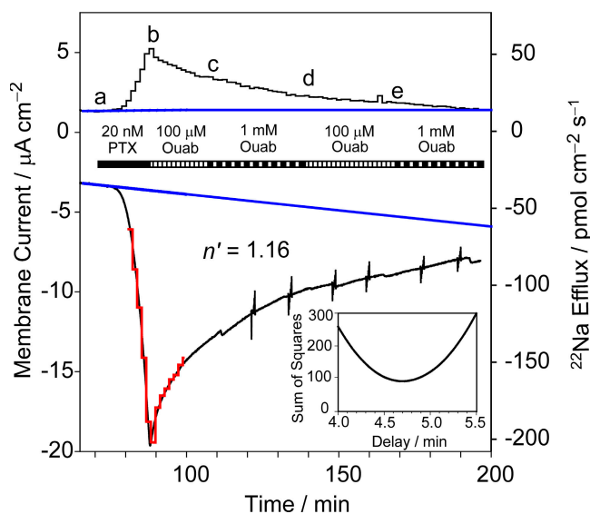
Figure 5. Determination of the flux ratio exponent n' for Na/K pump-channels opened by palytoxin. The axon was internally dialyzed with 98 mM Na + and superfused with 400 mM Na + , and held at 0 mV. Simultaneous measurements of unidirectional 22 Na + efflux (top trace) and net current (bottom trace) were used to estimate the flux ratio exponent n' for Na/K pump-channels opened by 20 nM palytoxin. The inset figure illustrates the procedure to account for the delay between current measurements and the fraction collector that collected radioactive samples. Least-squares fits of Eq. 1 to the current and flux data were repeated for successive 5-s increments of delay, to find the delay time that minimized the sum of squared deviations for the estimate of n' . In this experiment, a time delay of 4.70 min resulted in a minimum in the sum of squares and gave an estimate for n' of 1.16. Baseline values (blue lines) for 22 Na + efflux and net current were used to correct measured values in the determinations of n' . The red trace represents the measured efflux data transformed by Eqs. 1 and 2 using the best-fit n' and delay value obtained from the fits. In the presence of external Na + , saturating concentrations of ouabain fully reverse palytoxin-induced 22 Na + efflux in ~100 min. Vertical current displacements are in response to voltage staircases, with 0.5 mV steps, from -5 to 5 mV applied to monitor membrane conductance during the decline in current and flux.
