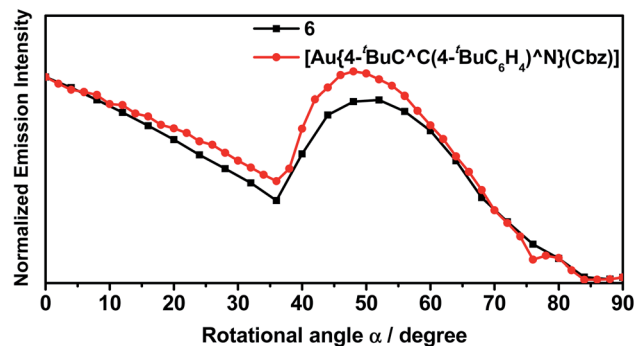
Fig. 6 Angular-dependent PL intensities of the p-polarized light of 6 and [\text{Au}\{4\text{-}^t\text{BuC}_6\text{H}_4\text{C}(4\text{-}^t\text{BuC}_6\text{H}_4)\text{N}\}(\text{Cbz})] (11% v/v) in m -CBP thin films with 20 nm thickness.
