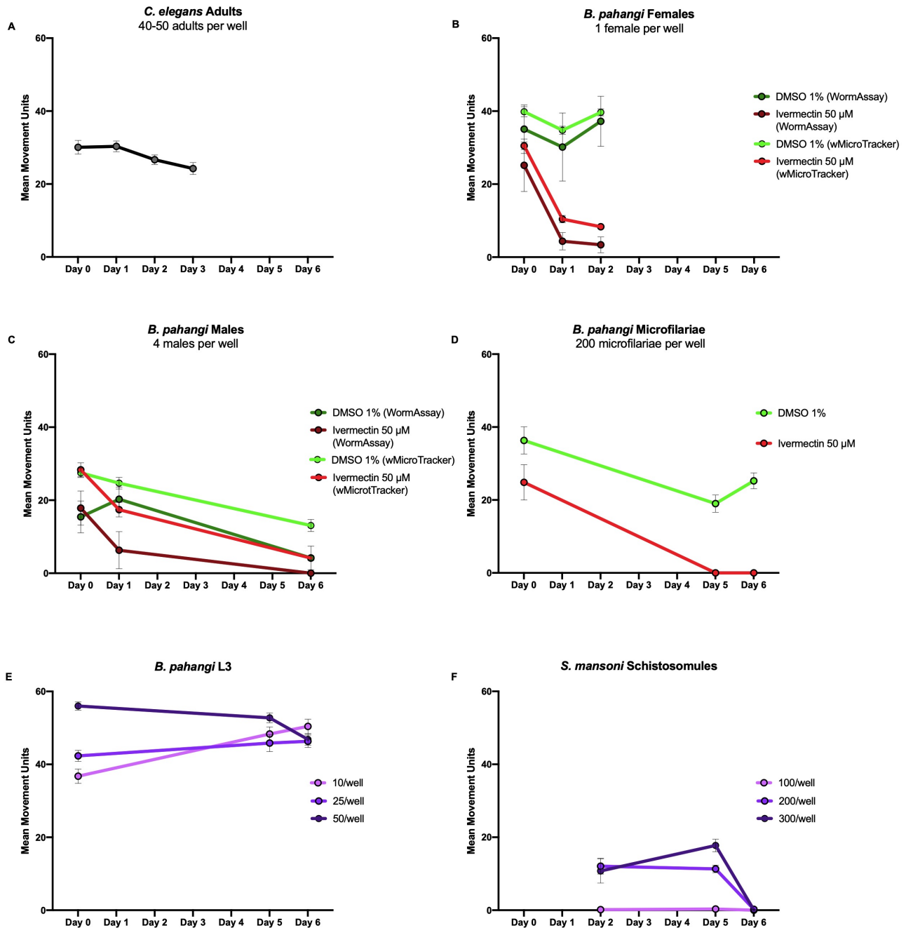
Figure 1: Results of motility screens of C. elegans adults (A) in the wMicroTracker, B. pahangi females (B) & B. pahangi males (C) in both the WormAssay and the wMicroTracker, and B. pahangi microfilariae (D), B. pahangi L3 (E) and S. mansoni schistosomules (F) in the wMicroTracker. Data are presented as mean \pm 95% CI.
