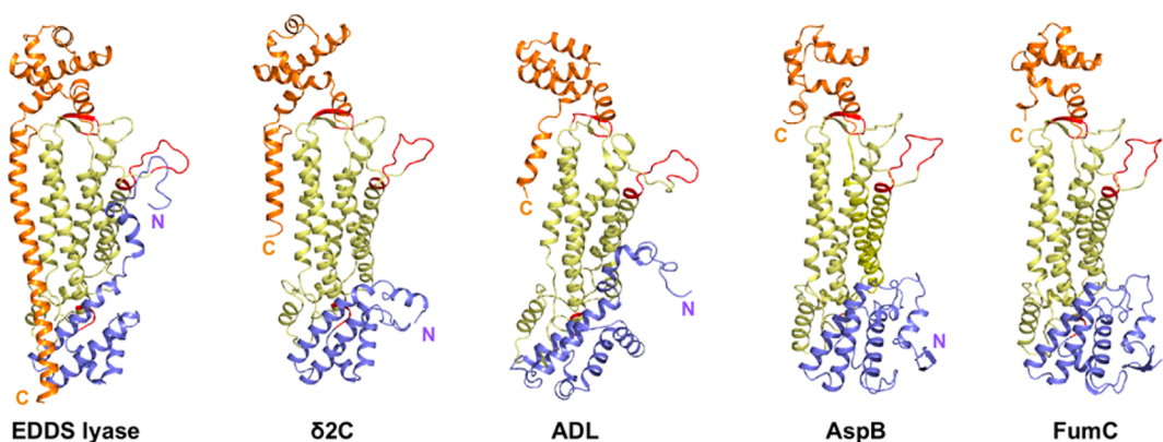
Figure 3. Comparison of the EDDS lyase monomer with other aspartase/fumarase superfamily enzymes. Cartoon representation of apo EDDS lyase (PDB entry 6G3D), argininosuccinate lyase ( \delta 2C, PDB entry 1HY1), adenylosuccinate lyase (ADL, PDB entry 2PTR), aspartase (AspB, PDB entry 3R6V), and fumarase (FumC, PDB entry 1YFE). The N-terminal domain, central domain, and C-terminal domain are colored blue, yellow, and orange, respectively. The conserved regions C1, C2, and SS loop are colored red. The locations of the N- and C-termini are also shown.
