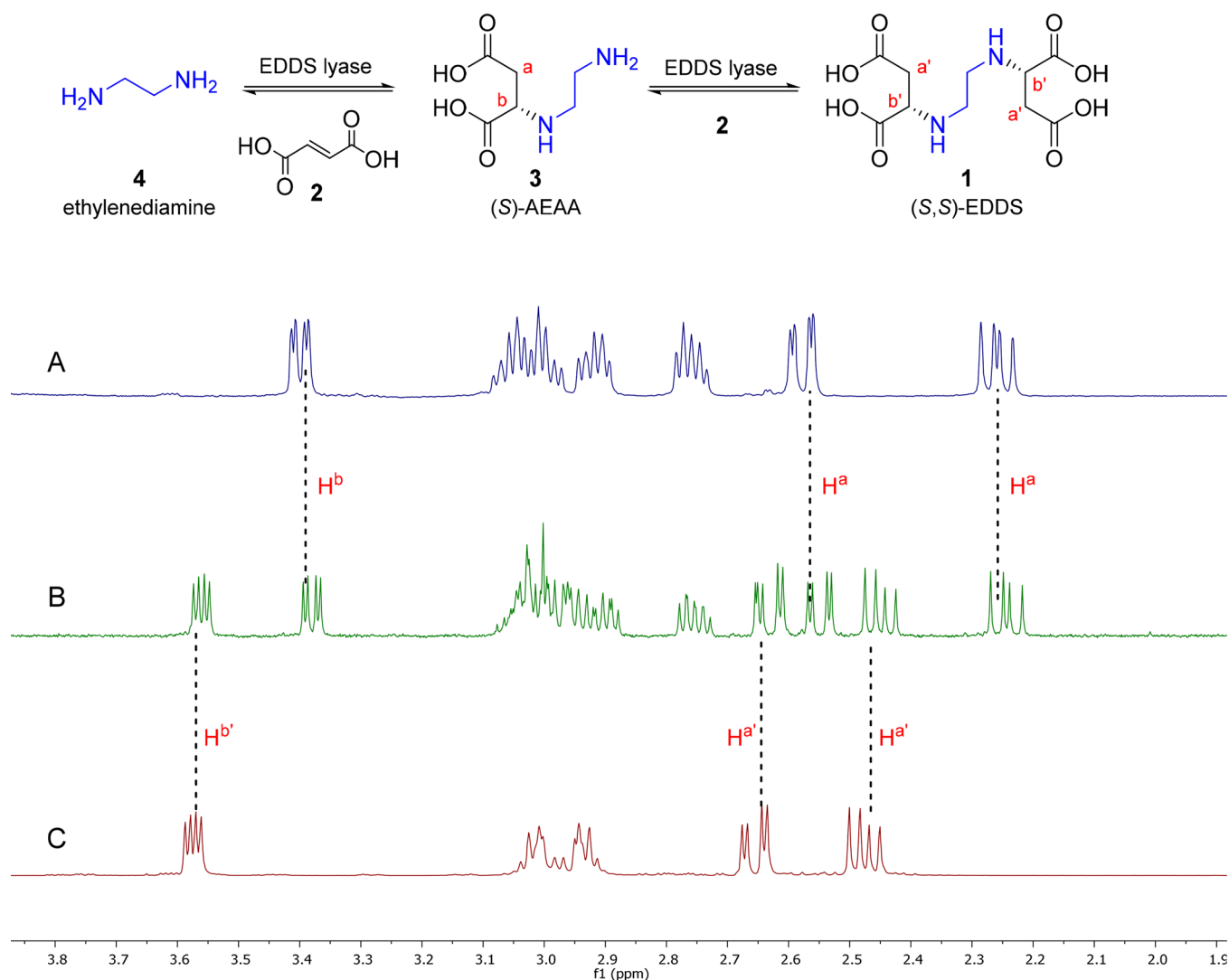
Figure 1. EDDS lyase-catalyzed addition of ethylenediamine (4) to fumaric acid (2) yielding AEEA (3) and EDDS (1). (A) 1 H NMR spectrum of AEEA (3) in D 2 O. (B) 1 H NMR spectrum of the reaction mixture after incubation for 24 h. The reaction was started by addition of EDDS lyase (0.05 mol %) to fumaric acid (50 mM) and ethylenediamine (10 mM) in 20 mM NaH 2 PO 4 -NaOH buffer (pH 8.5). (C) 1 H NMR spectrum of (S,S)-EDDS (1) in D 2 O. The assignments of key signals are highlighted in red.
