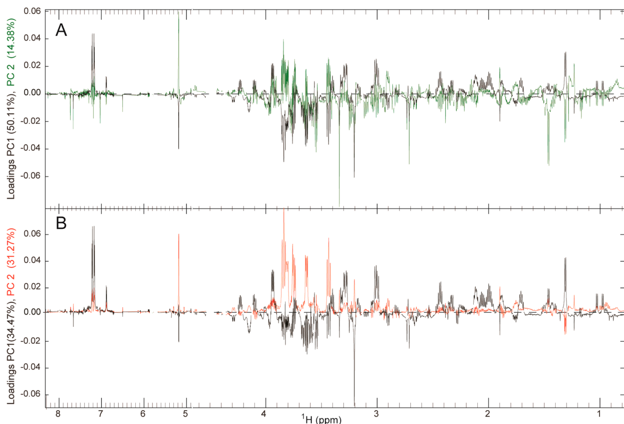
Figure 4. Loadings plots from the PCA analysis applied to (A) NMR spectra that have been normalized using PQN and (B) NMR spectra that have been normalized on the basis of the V_i/V_j dilution factor by VDTs prior to intragroup PQN. In each case PC1 is shown in black and PC2 in color (see Figure 5). Note chemical shift scale change at 5 ppm.
