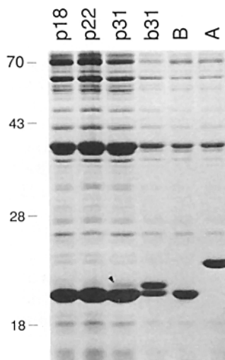
Figure 6. Coomassie blue-stained proteins of isolates from plasma (p) or brain (b) of a mouse sampled on days 18, 22, and 31 after inoculation with a clonal population of serotype B of B. turicatae . For comparison lysates of serotype B and A cells are in the rightmost two lanes. The samples from the plasma were purposefully overloaded with respect to the brain isolate. The arrow indicates a protein of 21 K in the lane of p31. This protein is in greater amounts in the b31 population. The acrylamide concentration was 12.5%. The migrations of molecular weight standards ( \times 1,000 ) are shown on the left.
