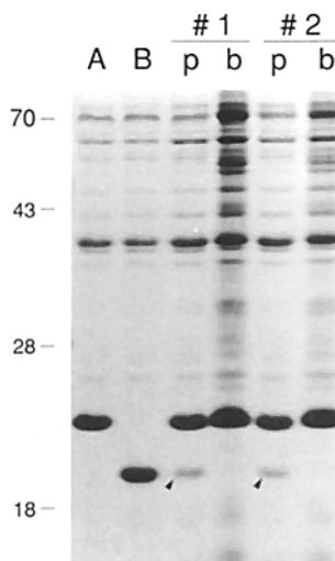
Figure 6. Coomassie blue-stained proteins of isolates from plasma (p) or brain (b) of a mouse sampled on days 18, 22, and 31 after inoculation with a clonal population of serotype B of B. turicatae . For comparison lysates of serotype B and A cells are in the rightmost two lanes. The samples from the plasma were purposefully overloaded with respect to the brain isolate. The arrow indicates a protein of 21 K in the lane of p31. This protein is in greater amounts in the b31 population. The acrylamide concentration was 12.5%. The migrations of molecular weight standards ( \times 1,000 ) are shown on the left.
