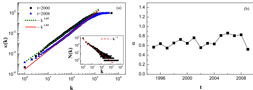
Figure 1 | Empirical preferential attachment to hot fields of new papers in the PR-PACS data set. (a) The cumulative probability functions \kappa(k) in the years 2000 and 2008. Inset: the distribution function of the sizes of fields. (b) The exponents \alpha for different years. We start our measurements from 1995, not 1976, the beginning year of the data, since the method requires a relatively large initial system. Notice \alpha = 0.52 – 0.87 is near the lower end of all the exponents collected in Table 1. The 2009 exponent is relatively smaller compared to its previous several years for reason that we do not yet know. If not mentioned, \Delta t is one year in this paper. The straight lines are guide to the eye through this paper.
