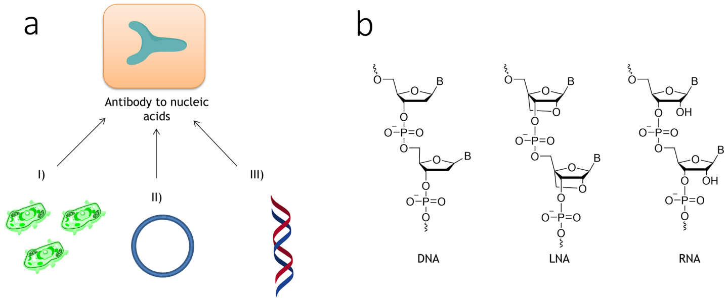
Fig 1. Current methods for the detection of a-DNA and chemical structures of nucleic acid antigens. (a) Current detection methods for anti-DNA: HEp-2 cell assay (I), ELISA using plasmid DNA antigen (II), and the novel assay suggested in this work (using synthetic DNA/LNA/RNA; III). (b) Chemical structures of DNA, LNA and RNA nucleotides.
