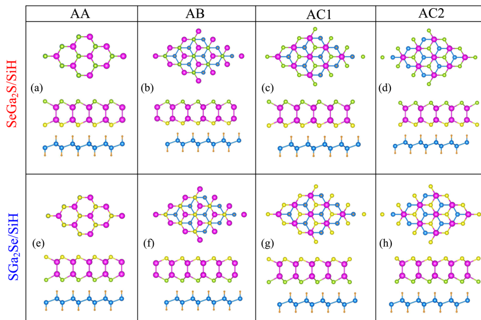
Fig. 2 Optimized atomic structures of the \text{SeGa}_2\text{S}/\text{SiH} heterostructure for different stacking patterns of (a) AA, (b) AB, (c) AC1 and (d) AC2 and optimized atomic structures of the \text{SGa}_2\text{Se}/\text{SiH} heterostructure for different stacking patterns of (e) AA, (f) AB, (g) AC1 and (h) AC2.
